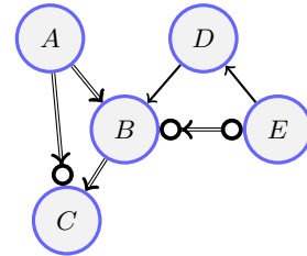
Figure 16: The ranking of KB from Figure 15, R , and the corresponding Bayesian Networks
